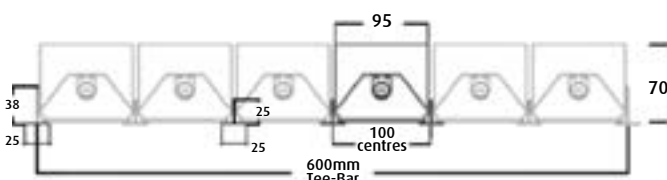
Position options along 600mm Tee-Bar
