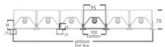
Position options along 600mm Tee-Bar
