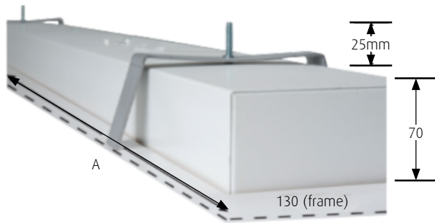
Mounting Screw / Detail
