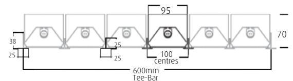
Position options along 600mm Tee-Bar
